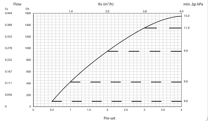
SIGMA Compact DN20 Low
