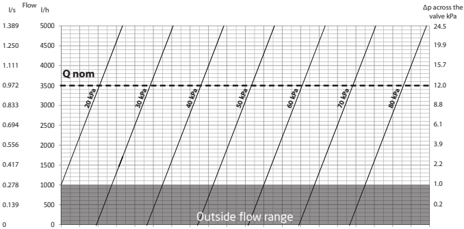
PV Compact DN32, 20-80 kPa
