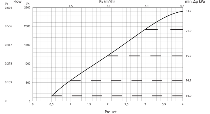
SIGMA Compact DN25 High
