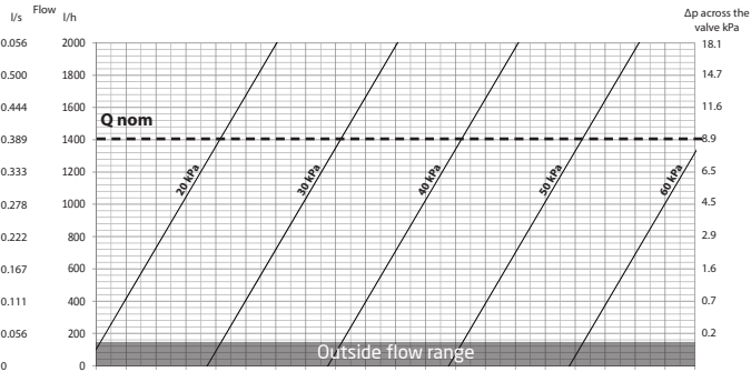
PV Compact DN20, 20-60 kPa
