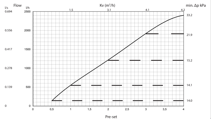
SIGMA Compact DN25 High
