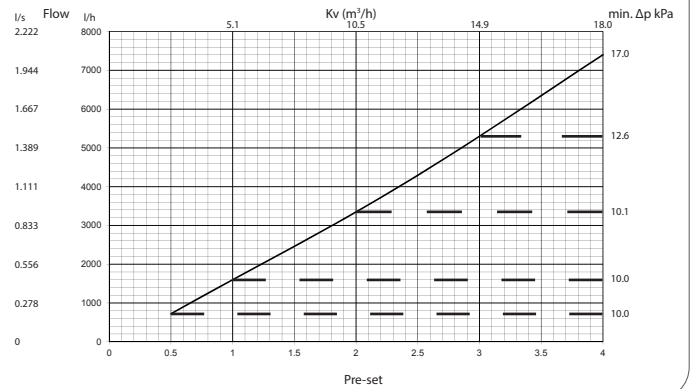
SIGMA Compact DN40
