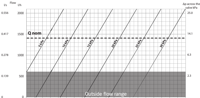
PV Compact DN25, 5-30 kPa
