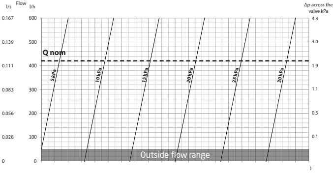
PV Compact DN15, 5-30 kPa
