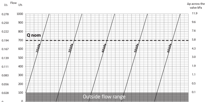
PV Compact DN15, 20-60 kPa
