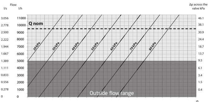
PV Compact DN50, 20-80 kPa
