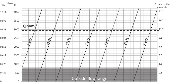
PV Compact DN25L, 20-80 kPa
