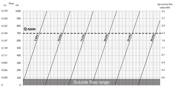
PV Compact DN20, 5-30 kPa
