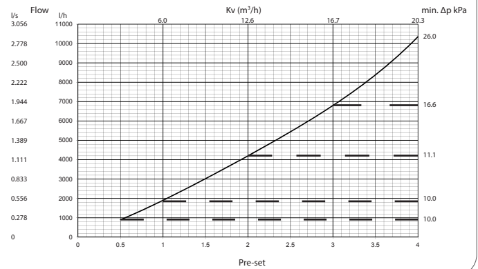
SIGMA Compact DN50
