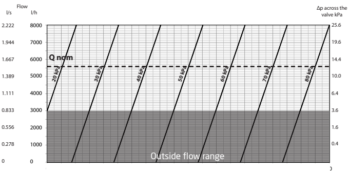
PV Compact DN40, 20-80 kPa
