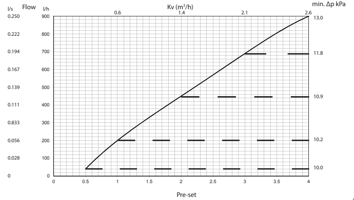
SIGMA Compact DN15 Low
